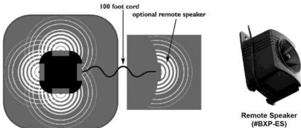
Diagram VI-a: Mounting Alternatives
